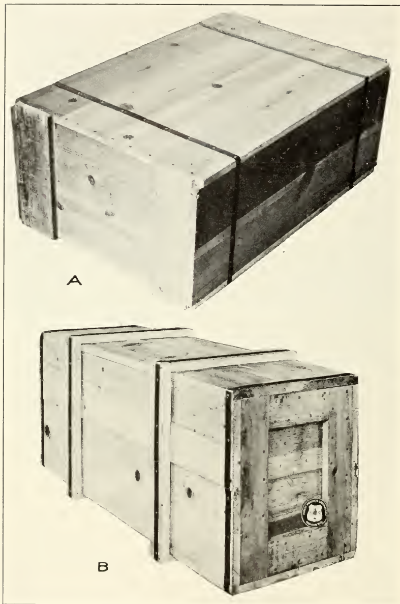
A, Nailed box reinforced with nailed straps placed away from the ends; B, a long box with battens and nailed metal straps. Such double reinforcing is desirable when straps alone will not give sufficient resistance to bending of sides, top, and bottom
